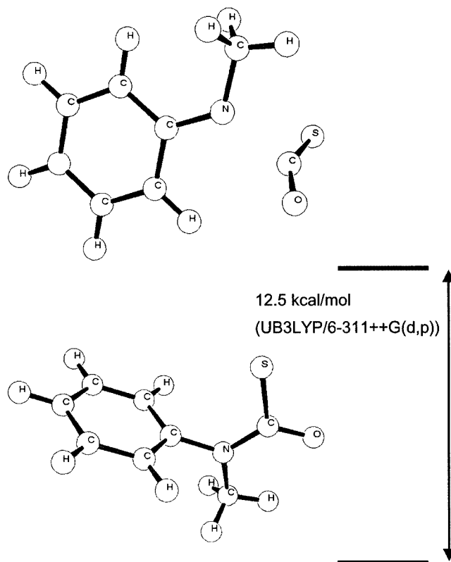
Figure 3. Structures of 1 and the transition state for the loss of calculated at the UB3LYP/6-311++G(d,p) level of theory
