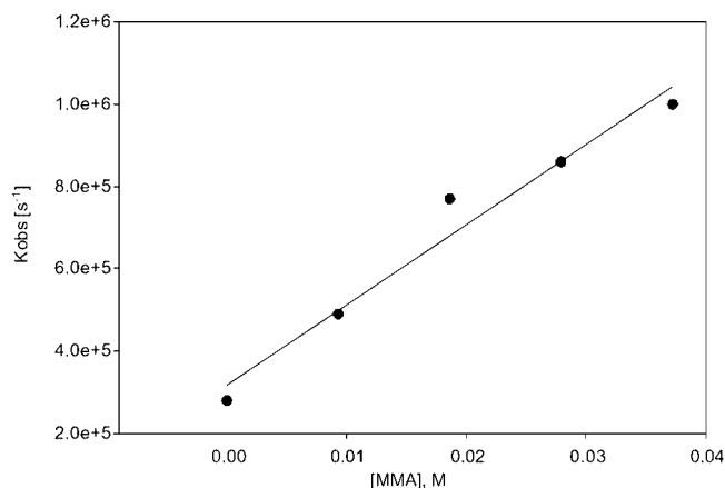
Figure 7. Decay rate of 1 in the presence of five different concentrations of MMA
