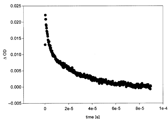
Figure 5. Transient decay trace, recorded at \lambda = 370 nm, upon laser flash photolysis ( \lambda_{\text{exc}} = 266 nm) of 4 in acetonitrile at ambient temperature
