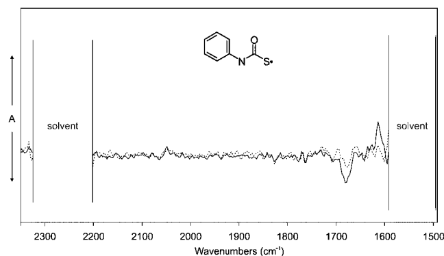
Figure 1. Time-resolved difference IR spectra (time resolution 500 ns, spectral resolution 6\text{ cm}^{-1} , spacer size 0.2\text{ m} ) showing the photochemistry of 4 in argon-purged acetonitrile; bands appearing on irradiation ( \lambda = 266\text{ nm} ) are pointing upwards, bands disappearing are pointing downwards; black: spectrum 500 ns after irradiation; dotted: spectrum after 20 \mu\text{s} .
