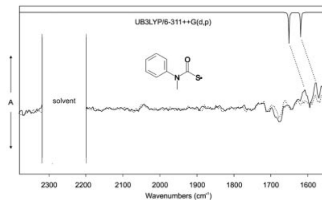
Figure 2. Top: calculated vibrational spectrum of 1 [UB3LYP/6-311+g(d,p), unscaled]; bottom: time-resolved difference IR spectra (time resolution 500 ns, spectral resolution 6 cm -1 , spacer size 0.05 mm) showing the photochemistry of 4 in argon-purged acetonitrile; bands appearing on irradiation ( \lambda = 266 nm) are pointing upwards, bands disappearing are pointing downwards; black: spectrum 500 ns after irradiation; dotted: spectrum after 20 \mu s
