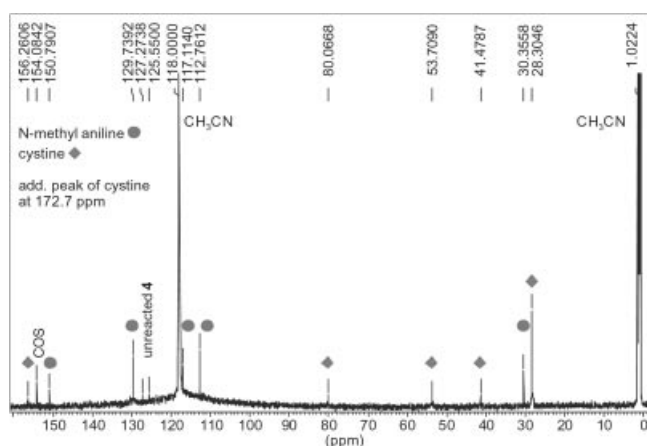
Figure 8. ^{13}\text{C} NMR spectra (150 MHz) after preparative photolysis (1 h, 266 nm, 10 Hz, 0.6 \text{ W s}^{-1} ) of 4 in degassed \text{CD}_3\text{CN} in a fused quartz NMR tube
