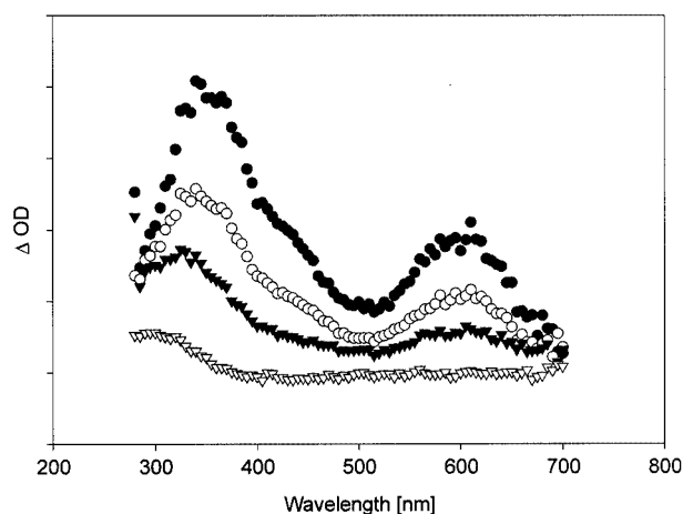
Figure 4. Time-resolved UV/Vis spectra [traces recorded after 1 \mu s (black dots), 5 \mu s (white dots), 17 \mu s (black triangles), and 75 \mu s (white triangles), spectral resolution 5 nm, cell size 1.0 cm] displaying the photochemistry of 4 in argon-purged acetonitrile
