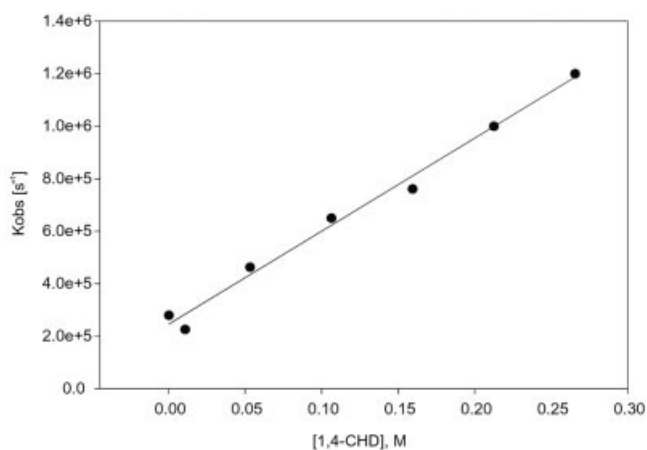
Figure 6. Decay rate of 1 in the presence of seven different concentrations of 1,4-cyclohexadiene
